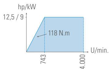
Broche ASA A2-5" – 4.000 rpm
