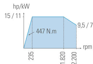
Broche ASA A2-8" – 2.200 rpm
